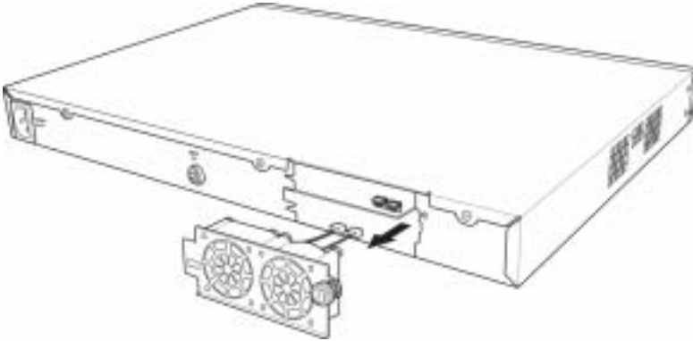
Figure 56. Detaching the fan from the module
